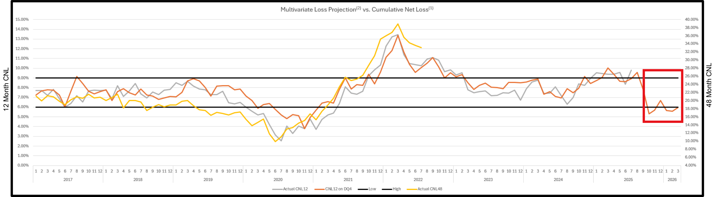
(Orange) Multivariate 12 Month CNL Model correlates to (Gray) Actual 12 Month CNL correlates to (Yellow) Actual 48 Month CNL
